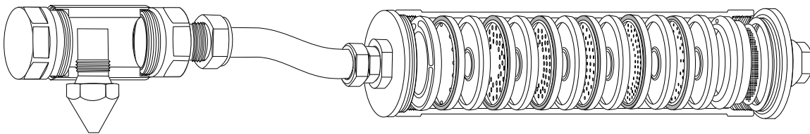
Cutaway of Cascade Impactor with Precutter
