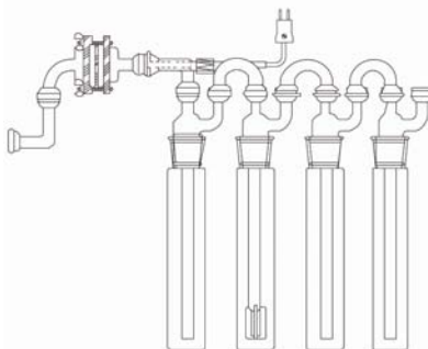
Basic Glassware Set (Assemble as Illustrated)
